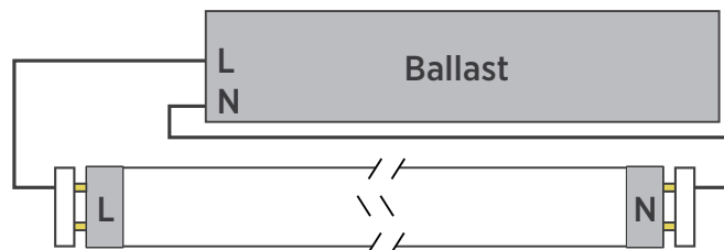
Dual-sided Type A Installation
