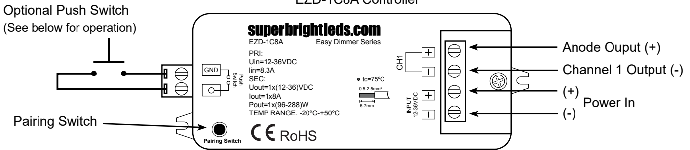
EZD-1C8A Controller
