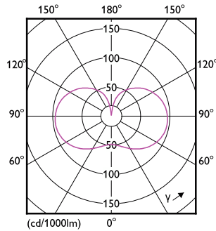
Light Distribution Diagram - 28GC/LED/840/ND E26 BB 6/1
