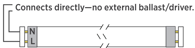
Single-sided Type B Installation
