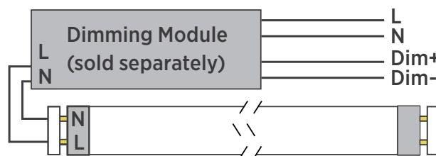
Single-sided Type B Installation (Dimming)
