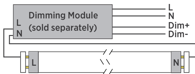
Dual-sided Type B Installation (Dimming)
