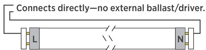
Dual-sided Type B Installation
