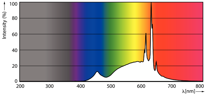
Spectral Power Distribution Colour - 8.5A19/LED/927/FR/P/ND 4/1FB
