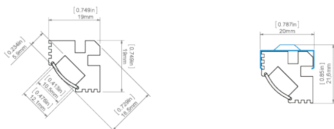
TAN-C5 extrusion and 45-STN mounting bracket
